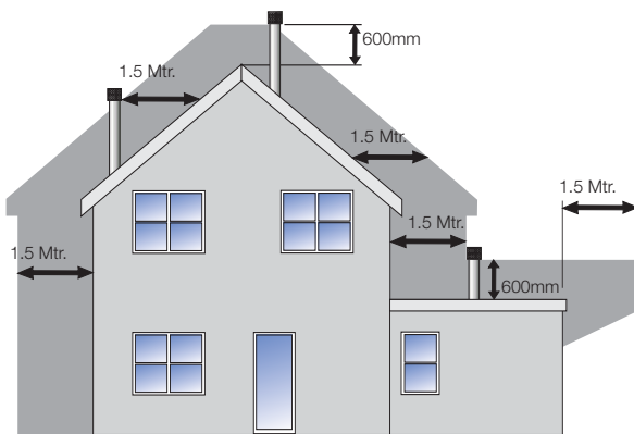
Fig. 15 Termination over gas appliance
