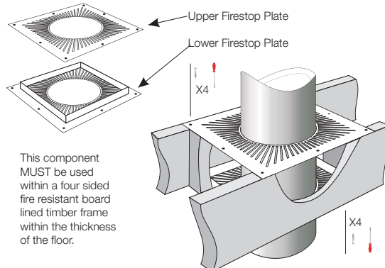
Fig. 4 Ventilated Firestop
