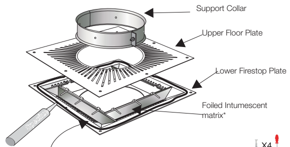
Fig. 3 Ventilated Ceiling Support
