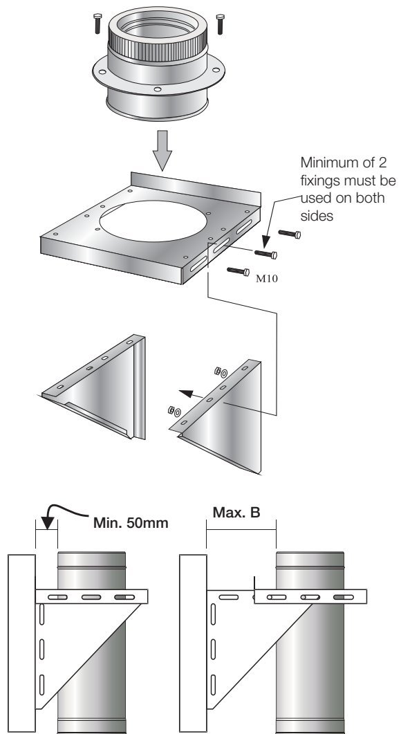
Fig. 9 Wall Support Assembly
