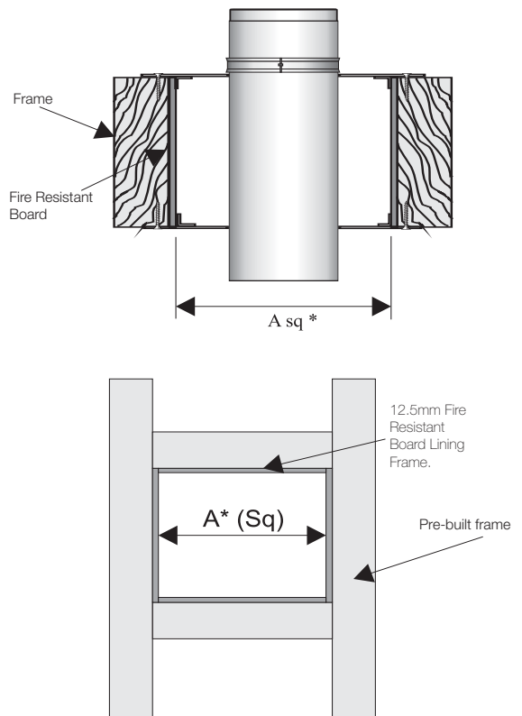
Fig. 6 Framing Data For Ventilated Components
