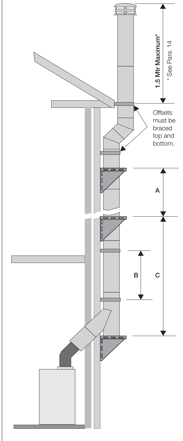
Fig 10 Support Components
