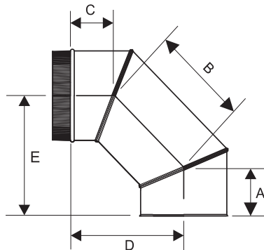
Dimensions for 90° and 85° Elbows
