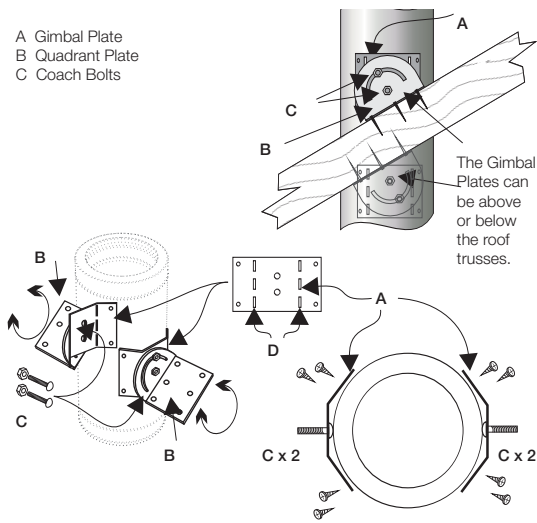
Fig. 8 Roof Support
