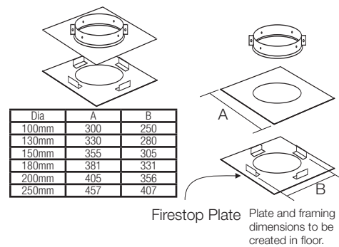
Fig. 7 Ceiling Support
