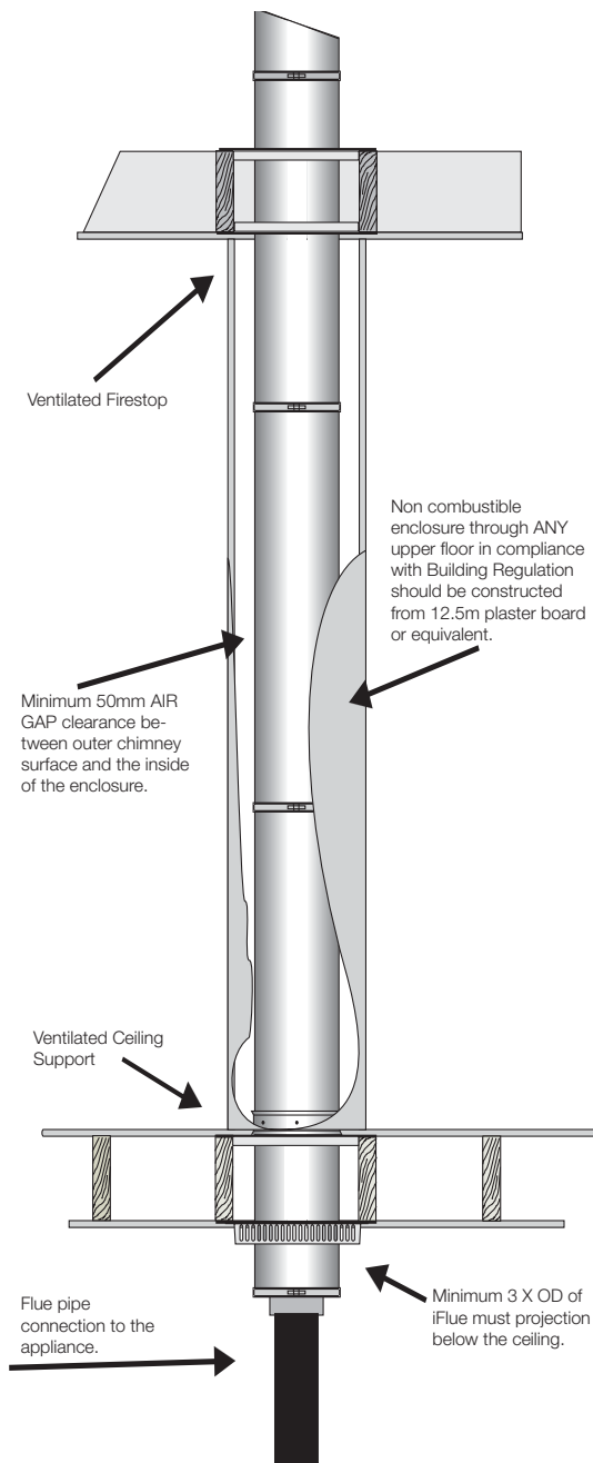
Fig. 5 Typical Configuration
