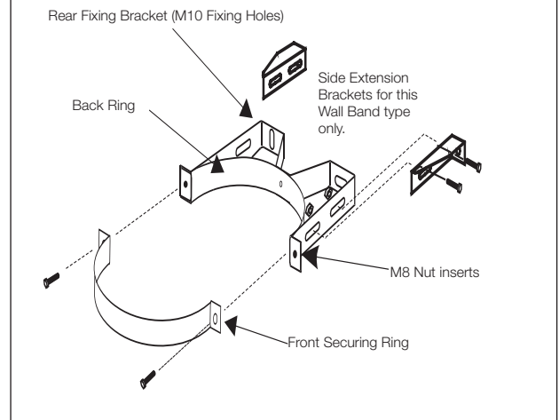
Fig. 12 Wall Band Extension Brackets
