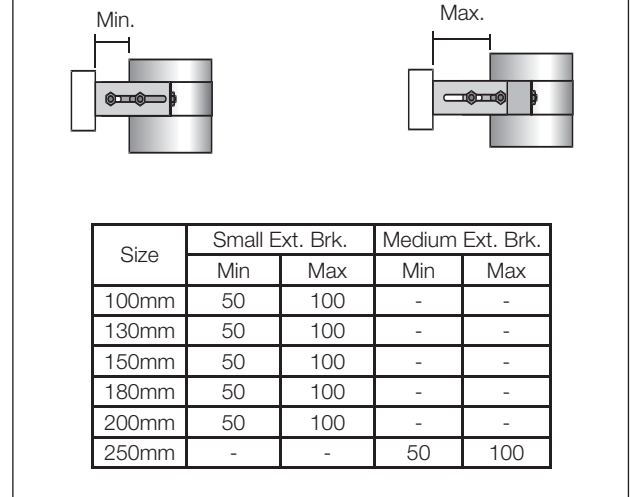
Fig. 12 Wall Band Extension Brackets
