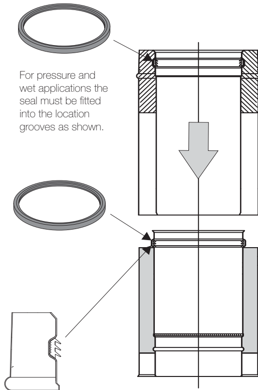
Fig. 2: Adjustable Length
