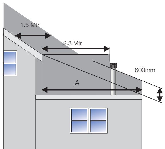
Fig. 18 Termination through an extension roof adjacent to a taller sloped roof building (Gas Appliances).
