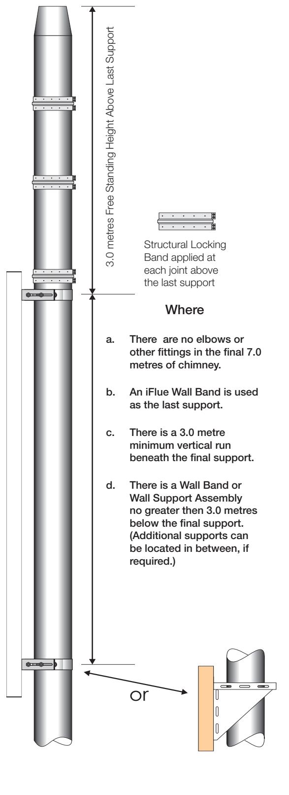
Fig. 13 Structural Locking Band positions
